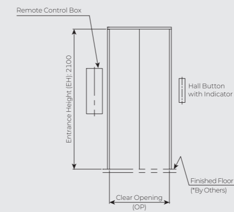
E050 TYPE WITH CP IN HOISTWAY
